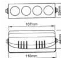
TL-L121R-12 TL-L121R-24
